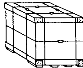
Figure 6: Fiber enclosed skid 1,000 lb and over
